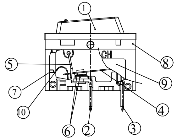
ASSEMBLE DRAWING
