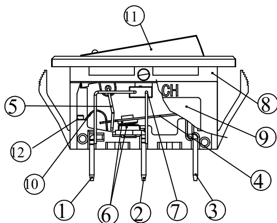
ASSEMBLE DRAWING
